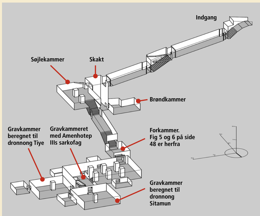
Fig. 7 Axonometrisk plan over KV 22, Dyn. XVIII, Amenhotep III (2/2) tegnet af Walton Chan © Theban Mapping Project. https://thebanmappingproject.com/sites/default/files/plans/KV22_2.pdf
